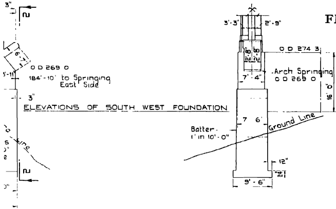
SIDE ELEVATION ON LINE 2-2
